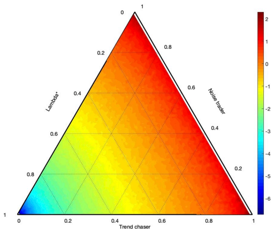
Fig. 3. Growth rate of \lambda^* investment strategy. We measure the expected growth of wealth over 20 periods for each combination of initial wealth across the three strategies.
